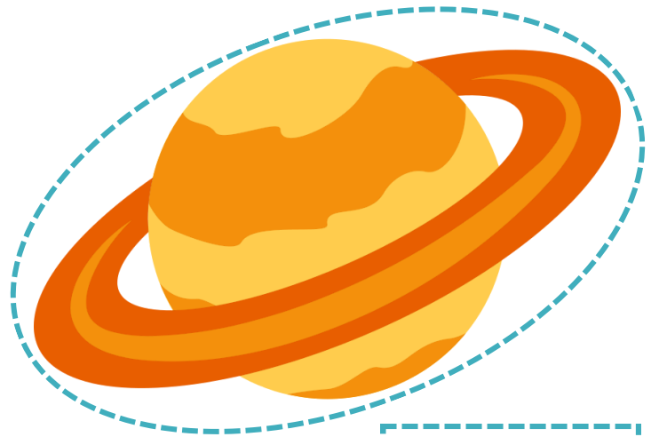
SATURN
